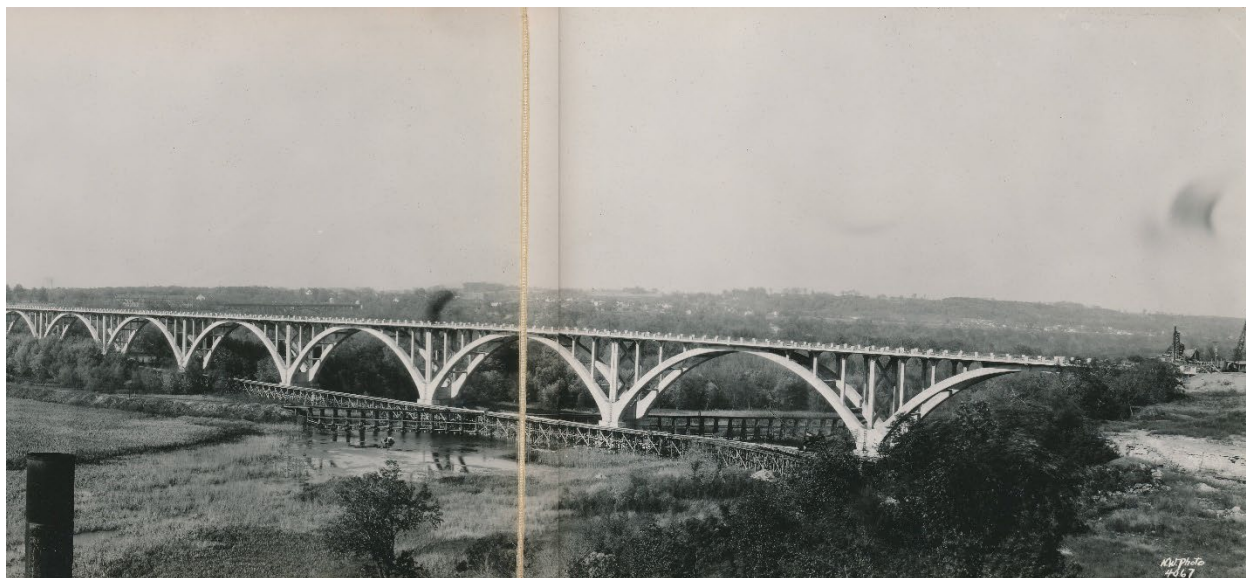
Figure 6. Newly constructed Mendota Bridge in 1926 by the Koss Construction Company from Pilot Knob (Holth 2013)
