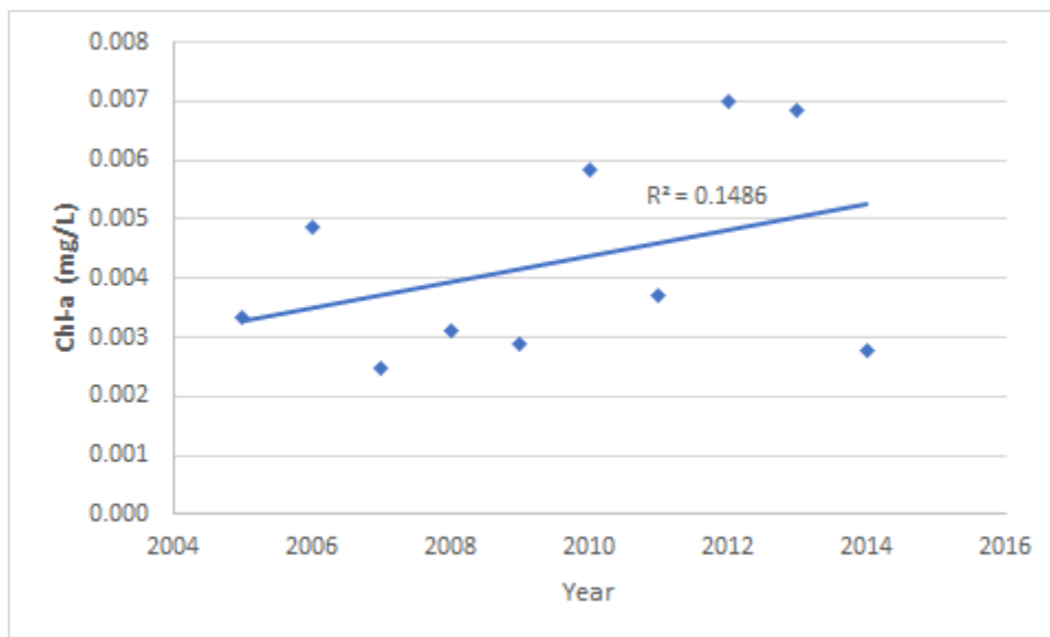
Chart 1-6: Fireman’s Lake Annual Average Chl-a Concentrations
